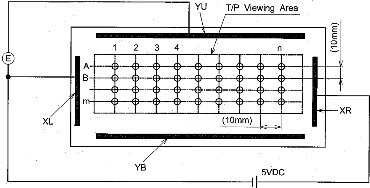
(b) Y axis linearity method , 100g VYU-VYB=5V , VOUT=VXR
