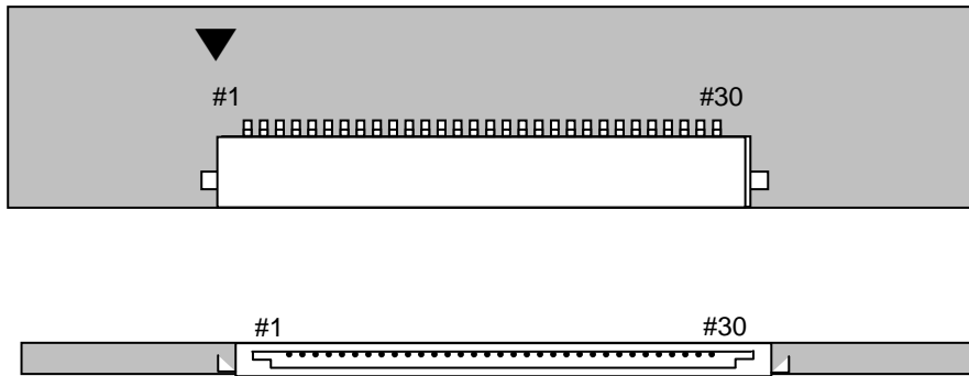
Fig. Connector diagram
