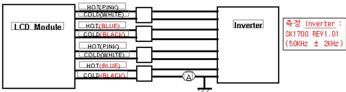
Fig. Measurement point of Lamp Current
