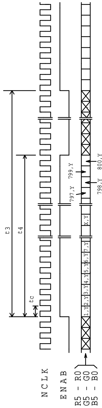
(2) Horizontal Timing
