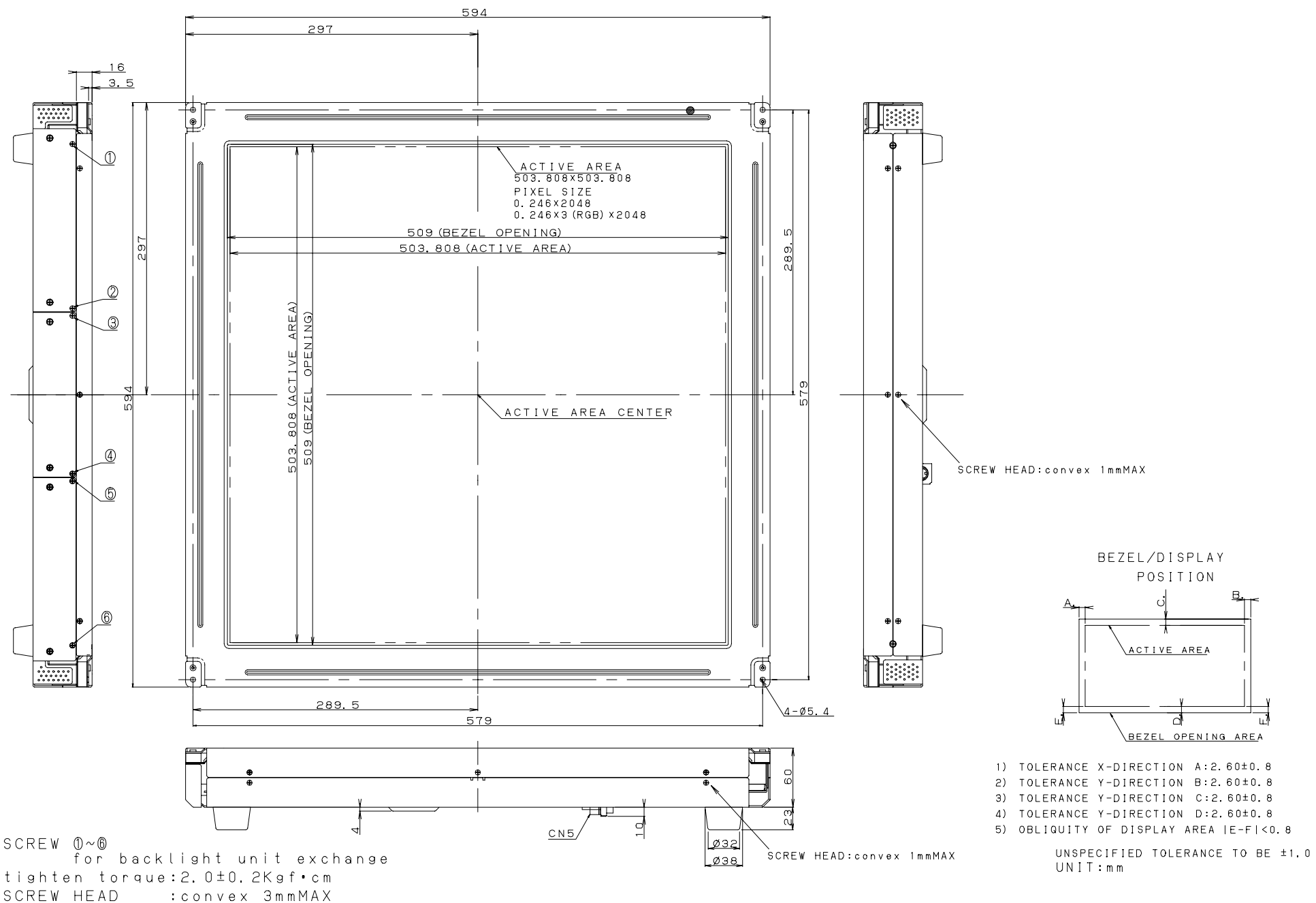
Fig. 4 LQ281L1LW11 MODULE OUTLINE 1/2
