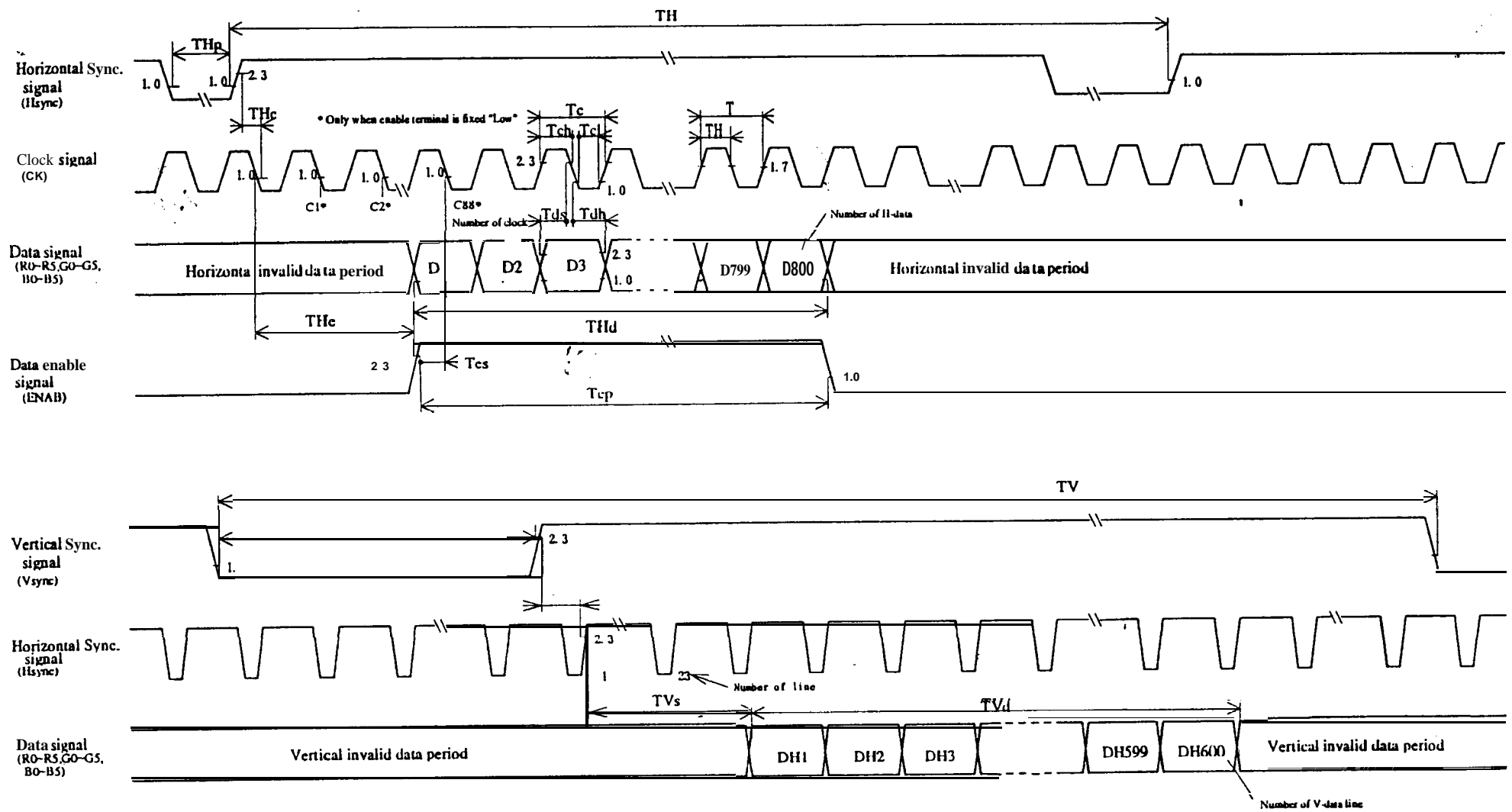
, Fig.2 Input signal waveform
