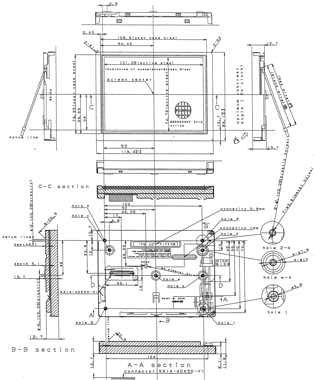
Fig.1 Outline Dimensions
