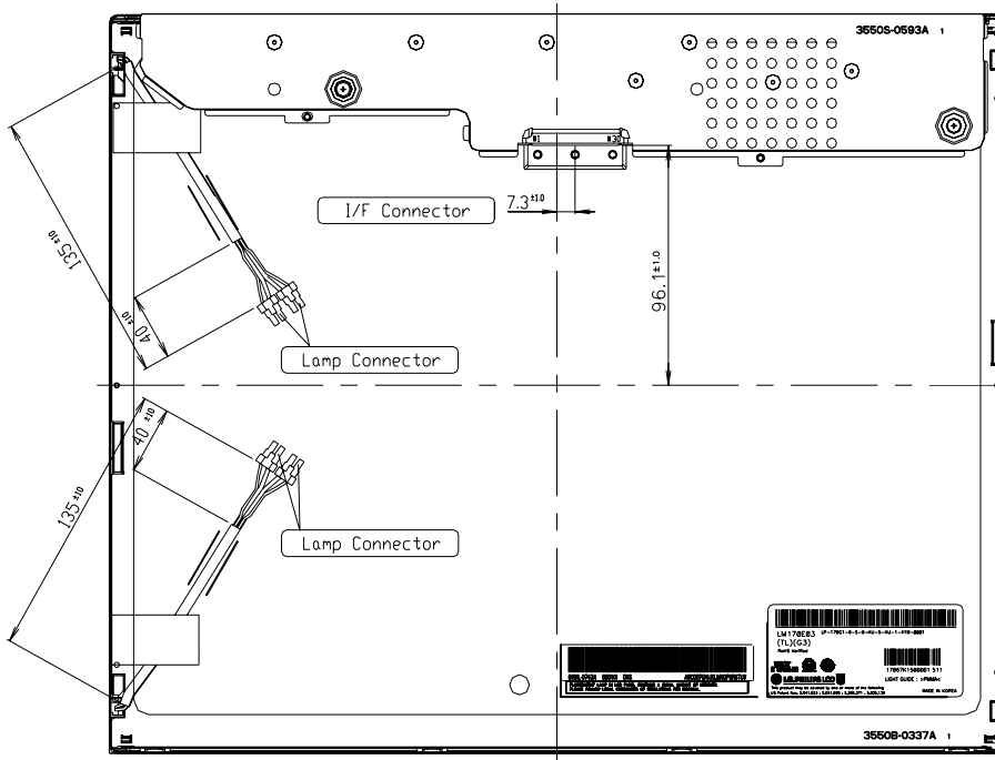
Figure 15. Rear view
