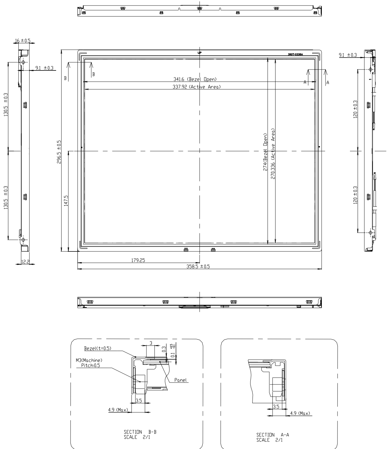
Figure 14. Front view
