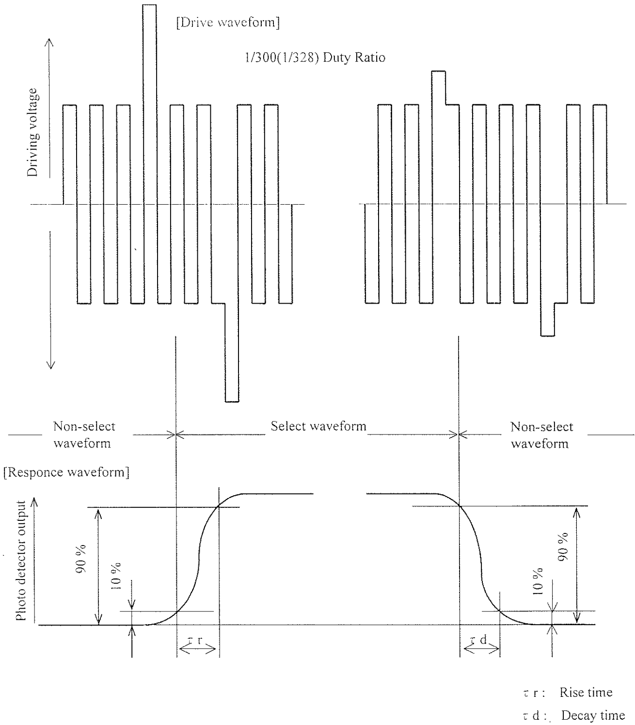
Fig.9 Definition of Response time
