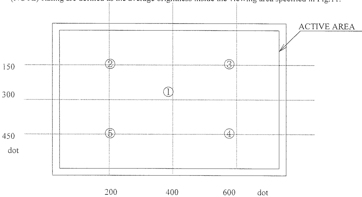
Fig.11 Measuring points (1-5)
