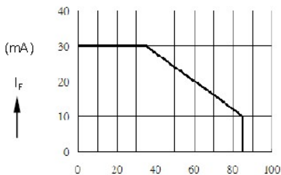
Ambient Temperature T A (°C) FORWARD CURRENT VS. AMBIENT TEMPERATURE
