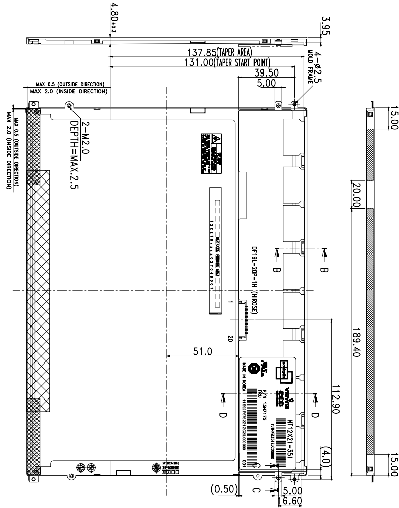
Figure 6. TFT-LCD Module Outline Dimensions (Rear View)
