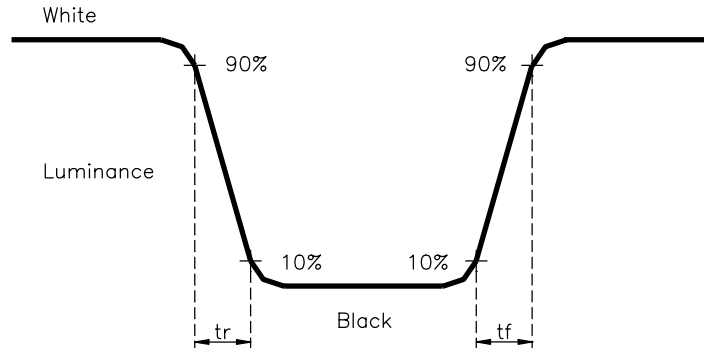
Fig.3 Definition of Response Time
