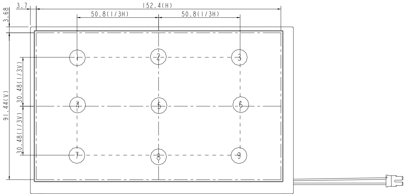
Fig8-1 Measuring point
