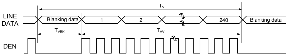
Vertical Timing Sequence
